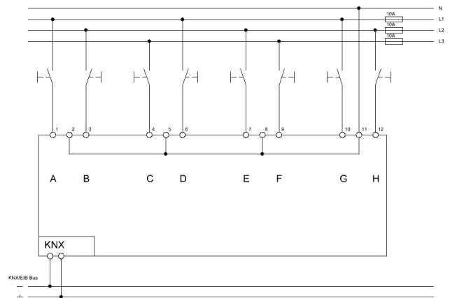
Exemplary circuit diagram BE-08230.02 - Different circuits
