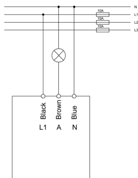
Exemplary circuit diagram RF-AKK1UP.01
