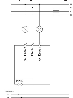
Exemplary circuit diagram AKU-02UP.03
