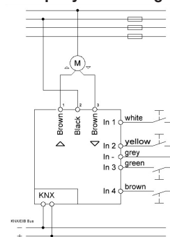
Exemplary circuit diagram AKU-B2UP.03
